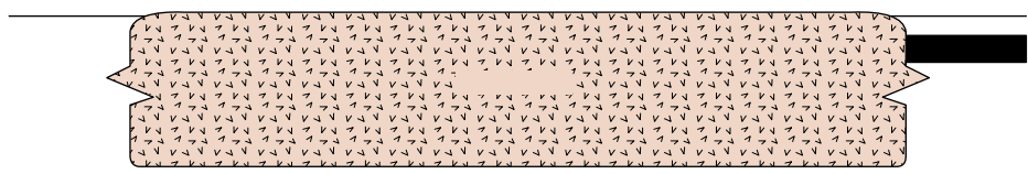
Stage A - Stable Continental Craton
