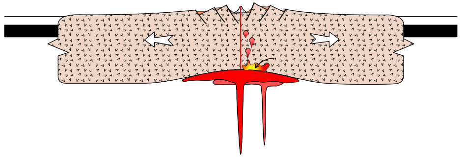
Stage B - Initial Rifting
