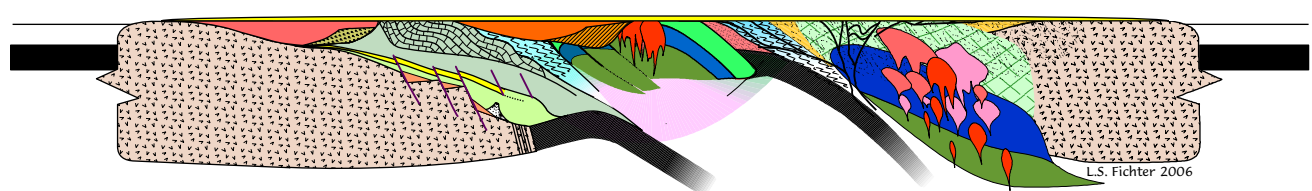
Stage I - Peneplained Continent
